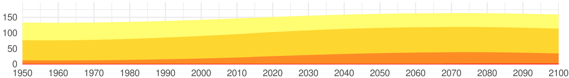
Moderating Emissions (SSP1-2.6)
