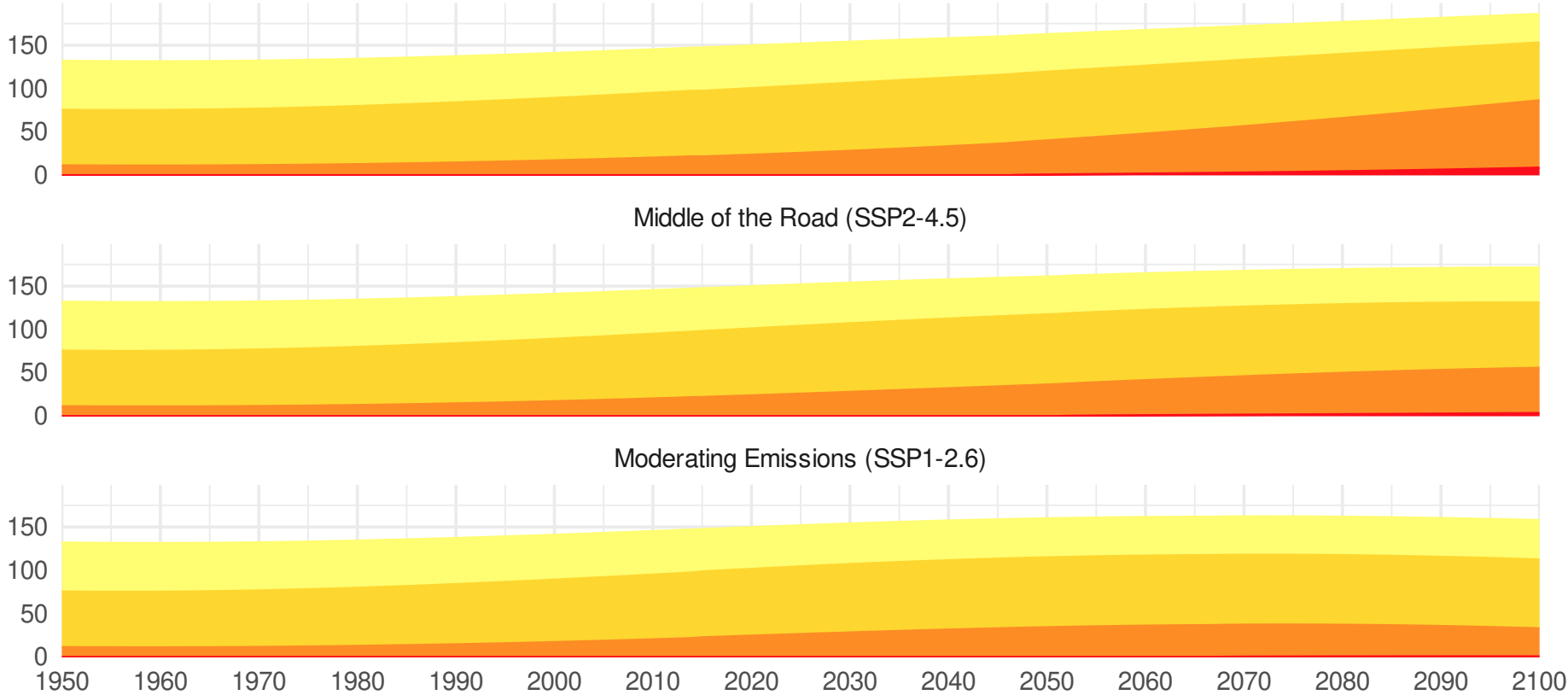
High Emissions (SSP3-7.0)
