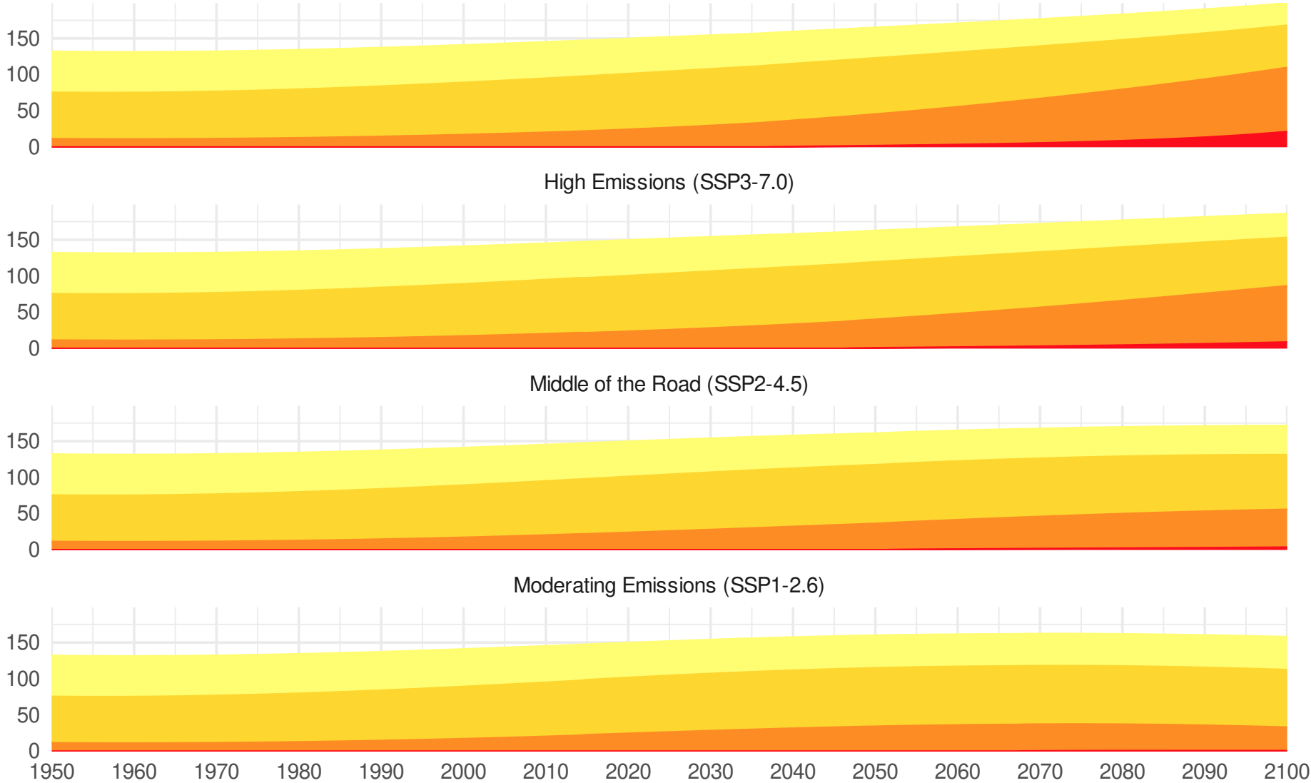
Accelerating Emissions (SSP5-8.5)
