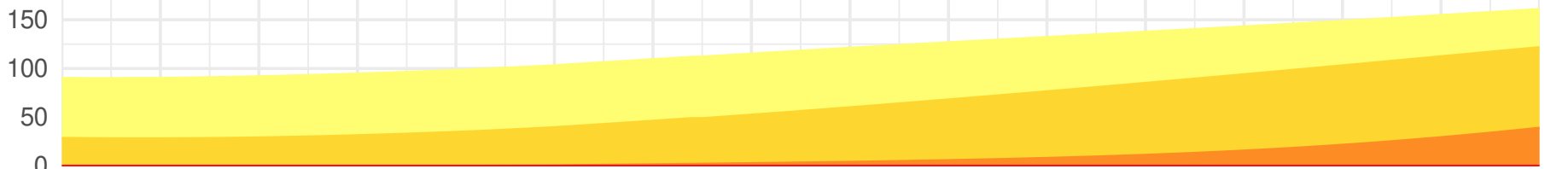
Middle of the Road (SSP2-4.5)
