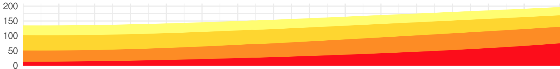
Middle of the Road (SSP2-4.5)
